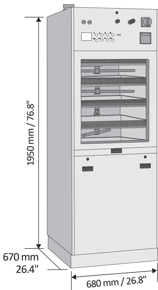
AWD655-10A Single door without boiler
