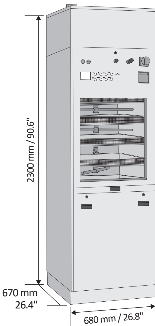
AWD655-10A-SC AWD655-10A-2SC Single door with boiler
